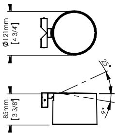
CM CORNER WALL-MOUNTING
